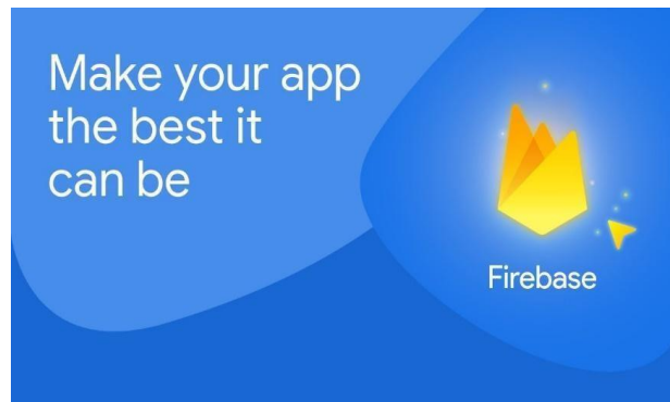
Figure 4. Firebase Software
