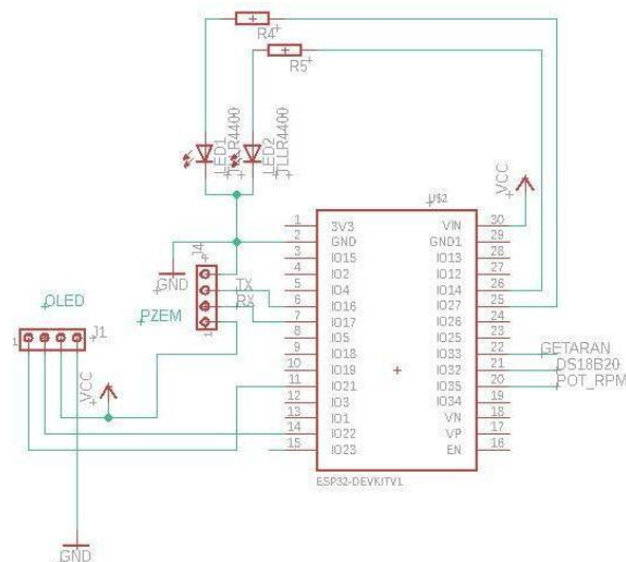
Figure 5. Complete Generator Parameter Measurement Circuit
